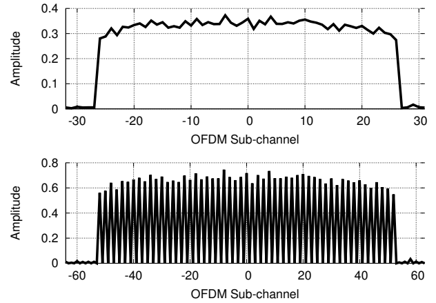
Figure 2—Creating a narrowband signal using WiSee: The first subplot shows the output of an FFT taken over an OFDM symbol. The second subplot shows the output of an FFT taken over two identical OFDM symbols. They show that taking a larger FFT over identical OFDM symbols, reduces each subchannel's bandwidth.
